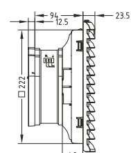
Fan and Filter CPF25
