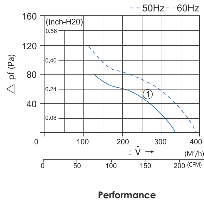
Fan and Filter CPF25
